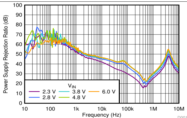
图 46. PSRR vs Frequency and V_{IN}
