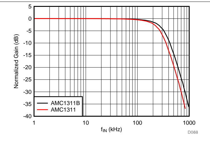
图 20. Normalized Gain vs Input Frequency
