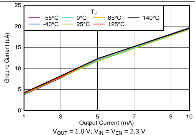
图 6. I_G vs I_{OUT} and Temperature for 1 mA to 10 mA
