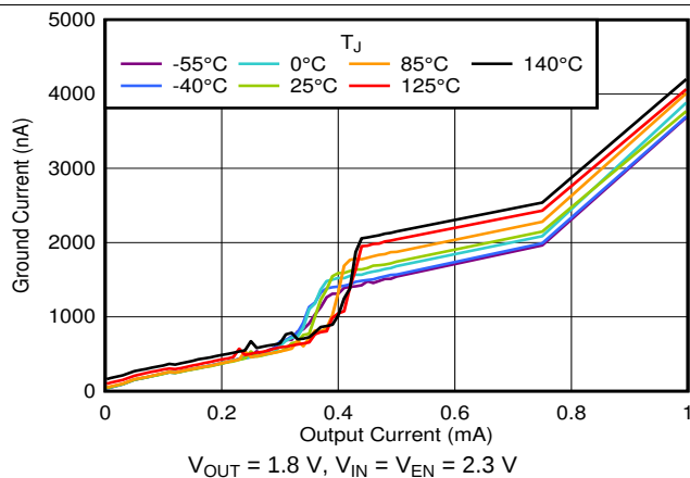
图 5. I_G vs I_{OUT} and Temperature Up to 1 mA
