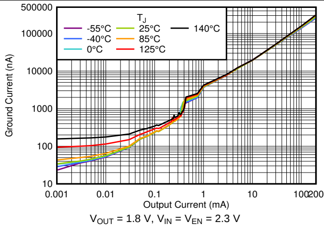
图 3. I_G vs I_{OUT} and Temperature up to 200 mA
