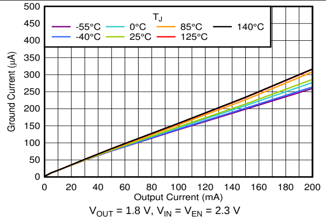
图 4. I_G vs I_{OUT} and Temperature Up to 200 mA
