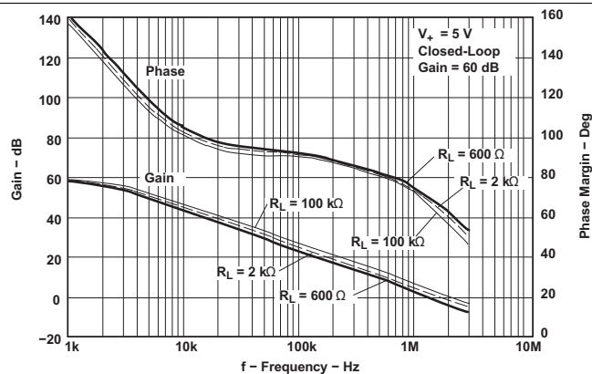
Figure 23. Gain and Phase Margin vs Frequency
