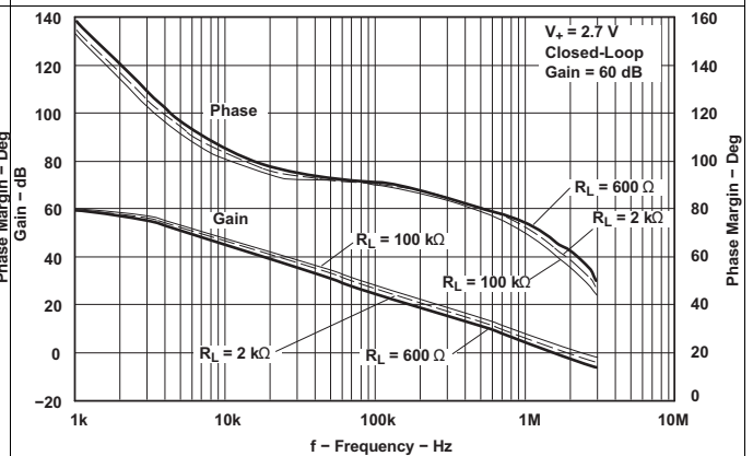
Figure 22. Gain and Phase Margin vs Frequency
