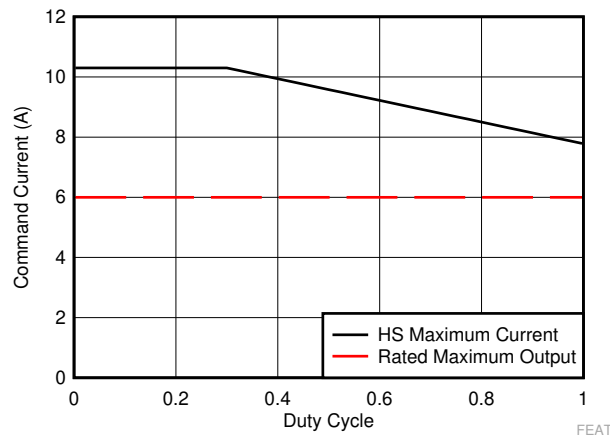
图 9-12. Maximum Current Allowed Through the HS FET - Function of Duty Cycle for LM61460-Q1
