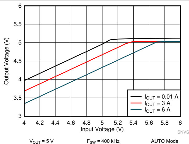
图 10-23. Dropout Curve
