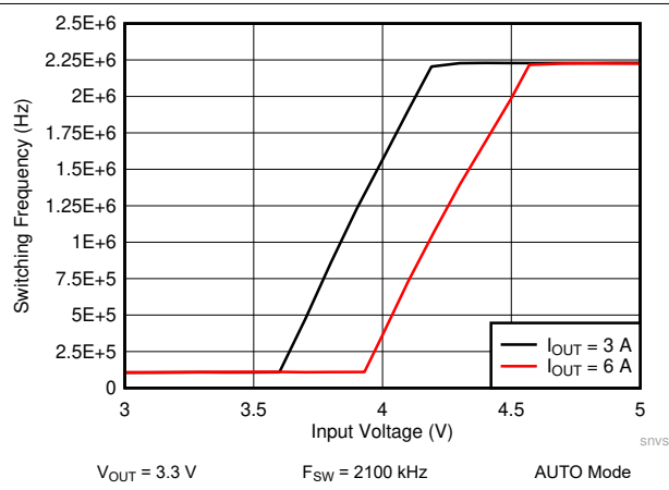
图 10-26. LM61460-Q1 Frequency Dropout Curve
