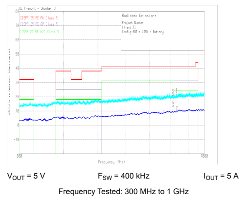
图 10-52. Radiated EMI Log Horizontal versus CISPR25 Limits
