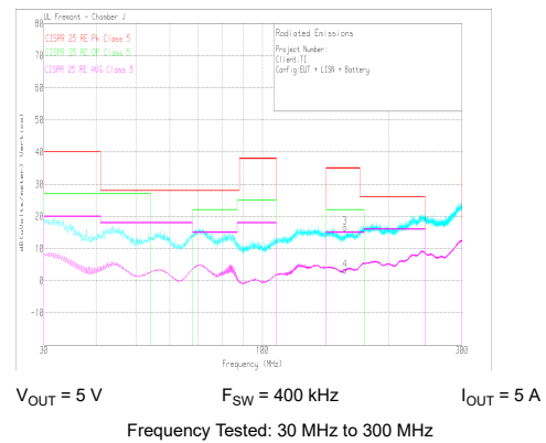
图 10-50. Radiated EMI Bicon Horizontal versus CISPR25 Limits
