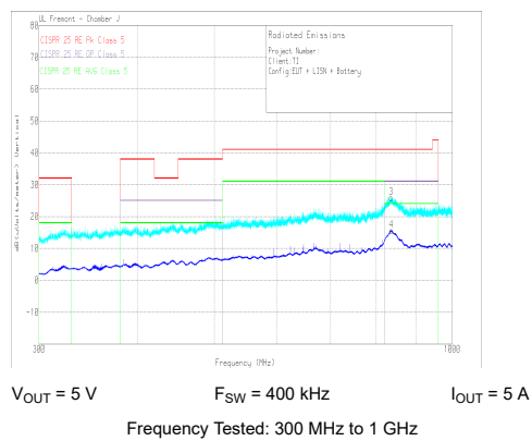
图 10-51. Radiated EMI Log Vertical versus CISPR25 Limits
