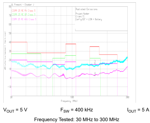
图 10-49. Radiated EMI Bicon Vertical versus CISPR25 Limits
