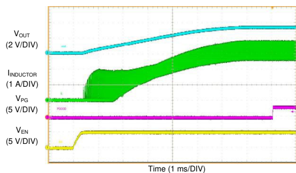
图 10-31. LM61460-Q1 Start-up with 50-mA Load
