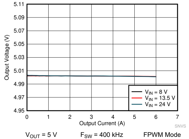
图 10-18. LM61460-Q1 Load and Line Regulation
