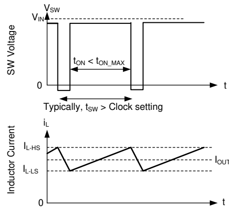
图 9-13. Current Limit Waveforms
