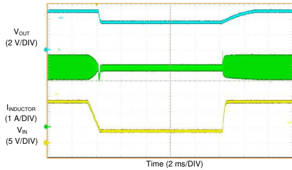
图 10-35. LM61460-Q1 Short Circuit Recovery
