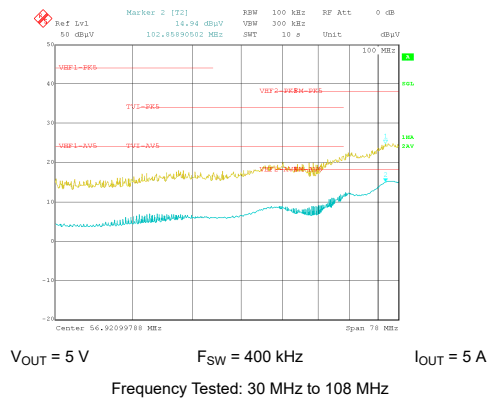
图 10-47. Conducted EMI versus CISPR25 Limits (Yellow: Peak Signal, Blue: Average Signal)
