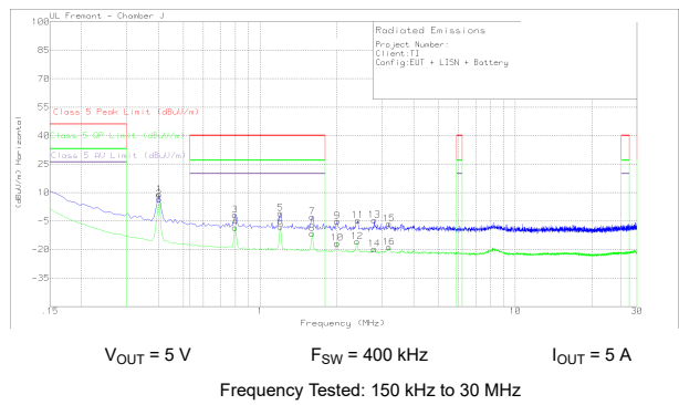
图 10-48. Radiated EMI Rod versus CISPR25 Limits
