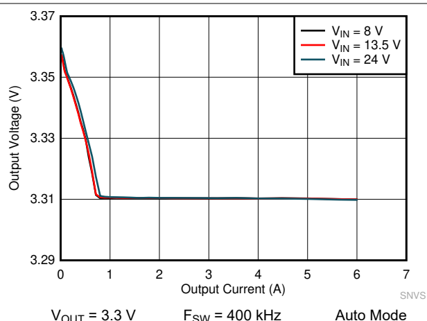
图 10-13. LM61460-Q1 Load and Line Regulation
