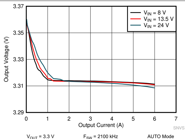
图 10-15. LM61460-Q1 Load and Line Regulation
