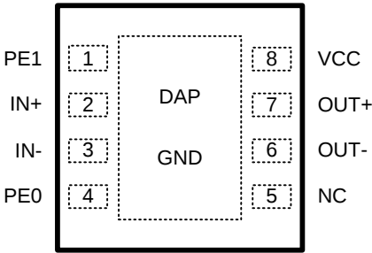
WSON Package
