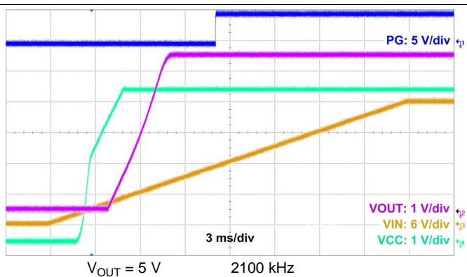
图 50. Start-Up Waveform
