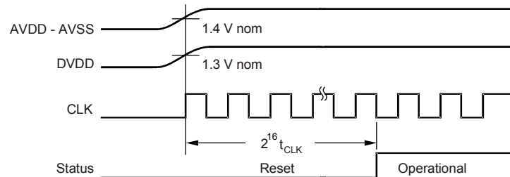
Figure 43. Power-On Sequence
