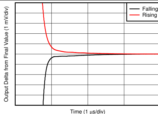
图 44. Settling Time
