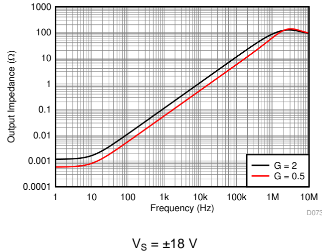
图 77. Closed-Loop Output Impedance vs Frequency
