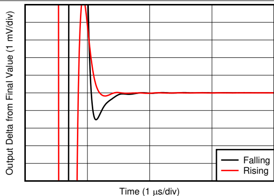
图 43. Settling Time
