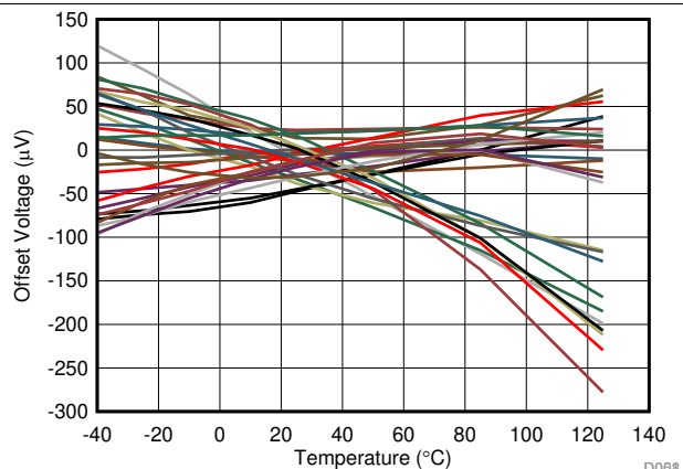
图 8. Output Offset Voltage vs Temperature
