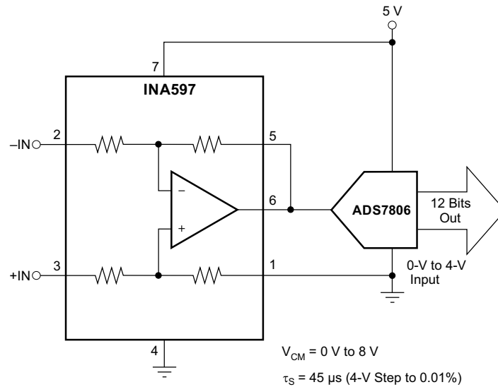
图 81. Differential Input Data Acquisition
