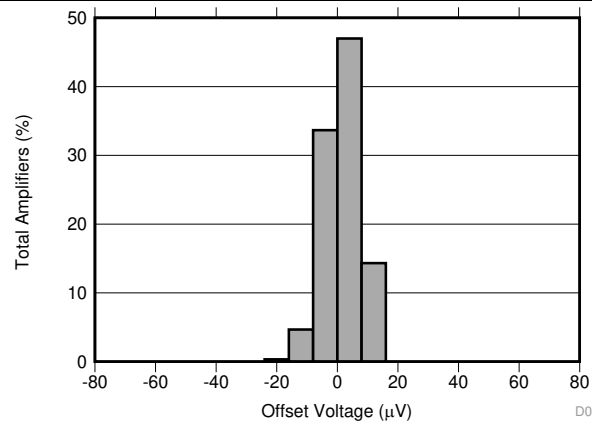
图 2. Typical Distribution of Offset Voltage (RTO)
