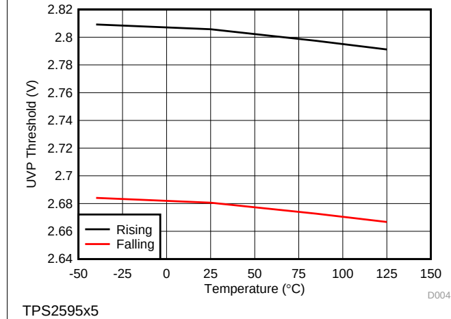
图 5. UVP Threshold vs Temperature
