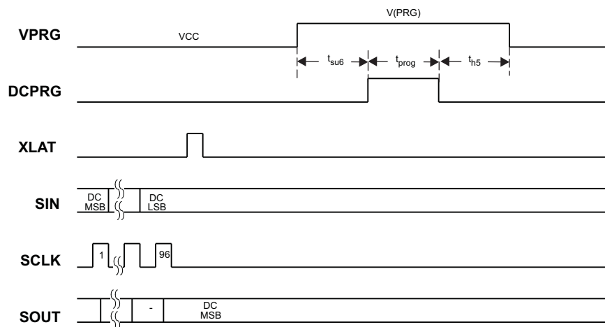
Figure 16. EEPROM Programming Timing Chart
