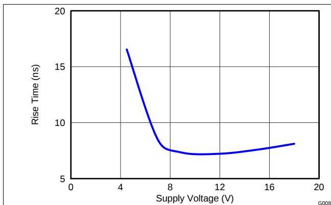
图 17. Rise Time vs Supply Voltage
