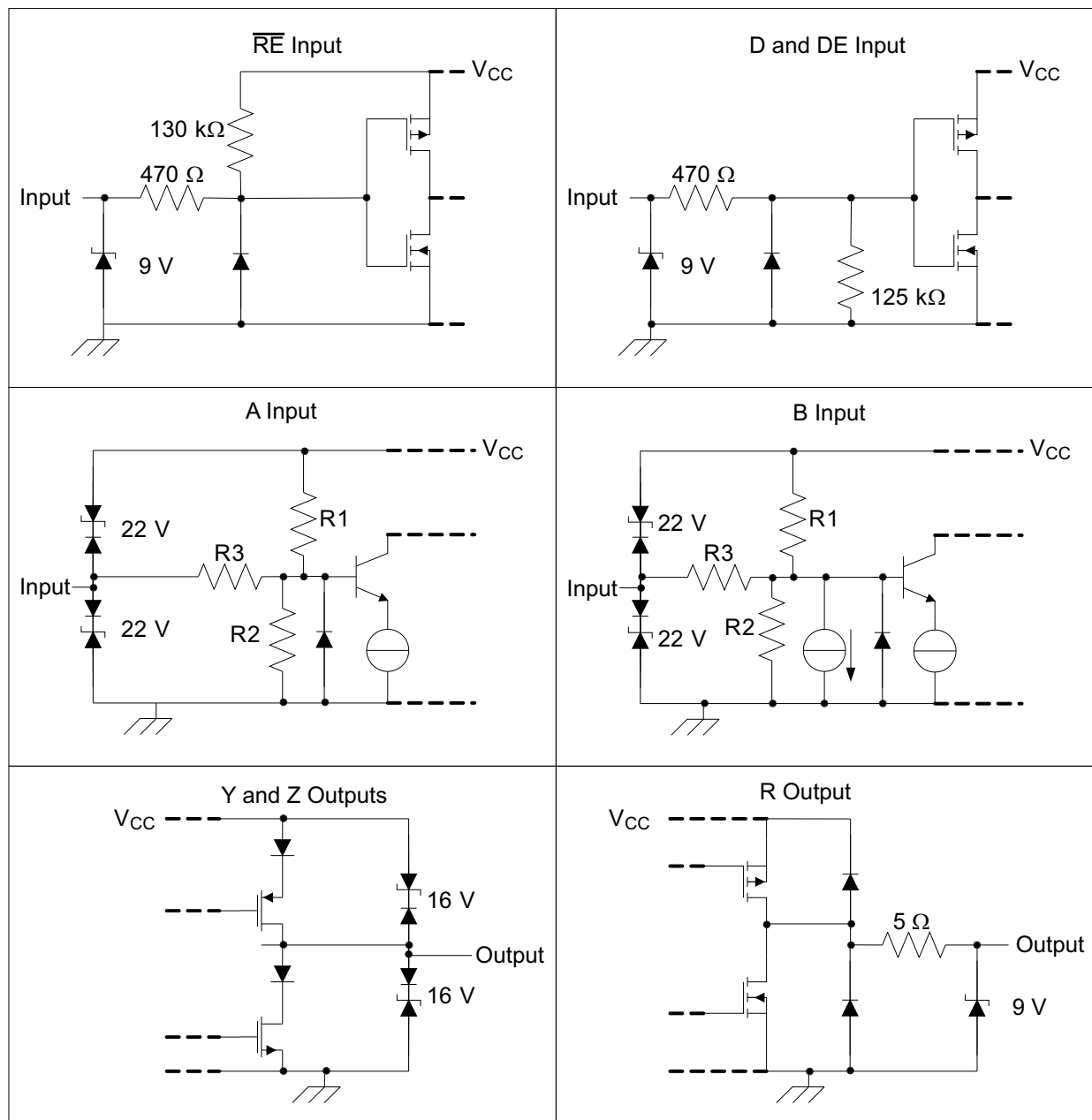
Figure 33. Equivalent Input and Output Schematic Diagrams
