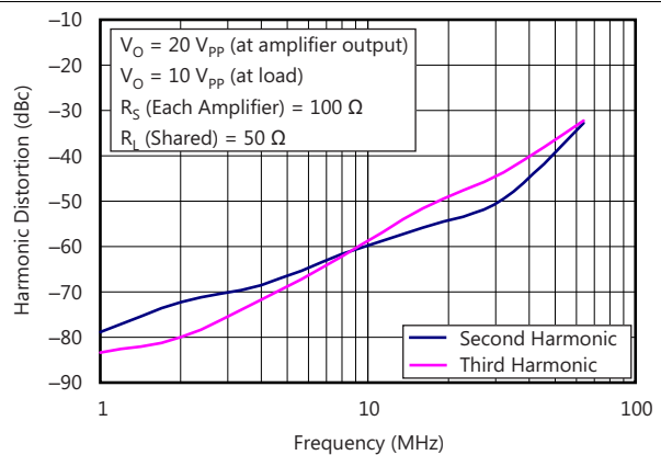
Figure 77. Harmonic Distortion vs Frequency, Two THS3091 Amplifiers in Load Sharing Configuration
