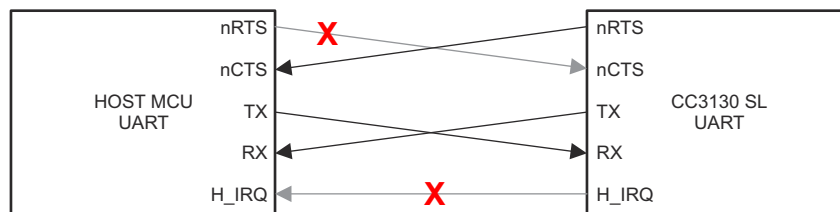
图 8-20. 3-Wire UART Topology
