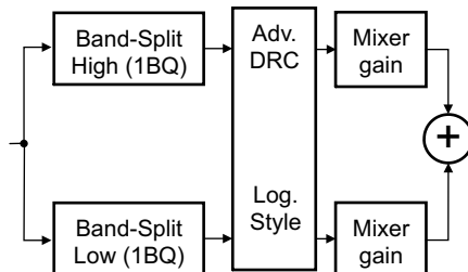
Figure 78. Dynamic Range Control
