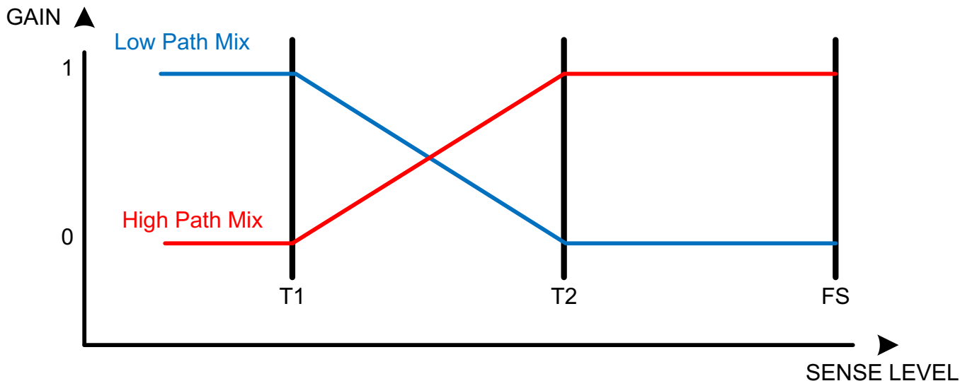
Figure 77. Dynamic Mixing
