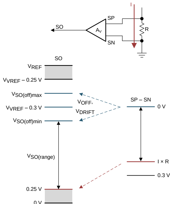
图 34. Unidirectional Current-Sense Regions
