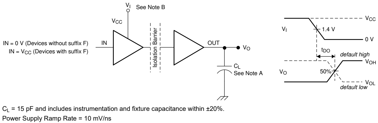
图 7-2. Default Output Delay Time Test Circuit and Voltage Waveforms
