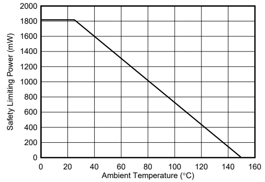
图 6-2. Thermal Derating Curve for Safety Limiting Power for DW-16 Package
