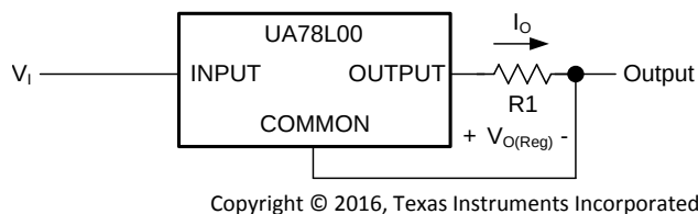
Figure 10. Current Limiter Example
