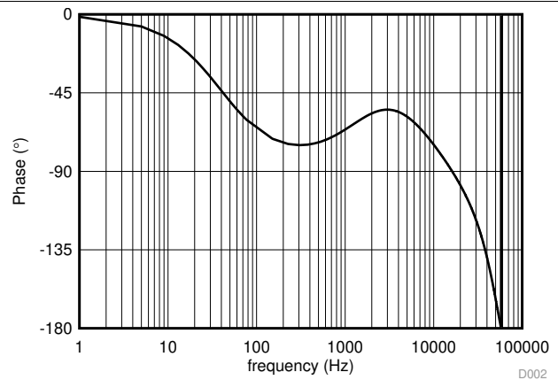
Figure 32. Converter Open-Loop Bode Plot - Phase
