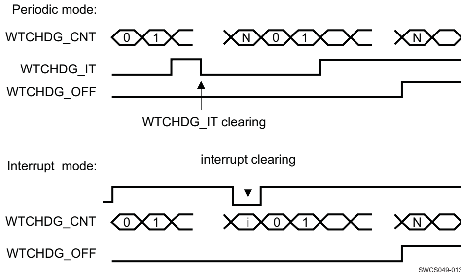
图 18. Watchdog Signals
