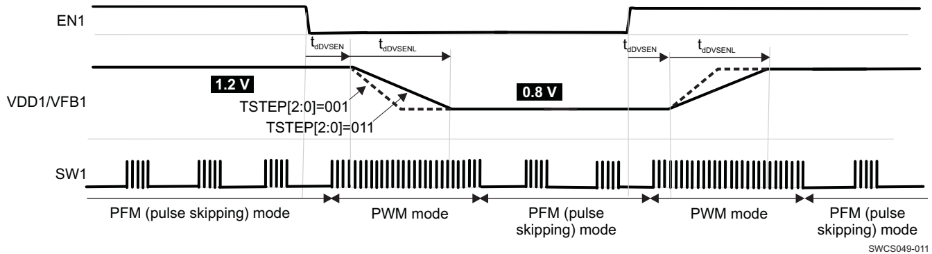
图 7. VDD1 Supply Voltage Control Through EN1
