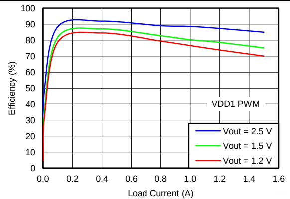
图 11. VDD1 Efficiency vs Load Current, 25°C, V_{IN} = 4 V, PWM
