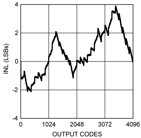
Figure 5. INL at V_A = 3 \text{ V}
