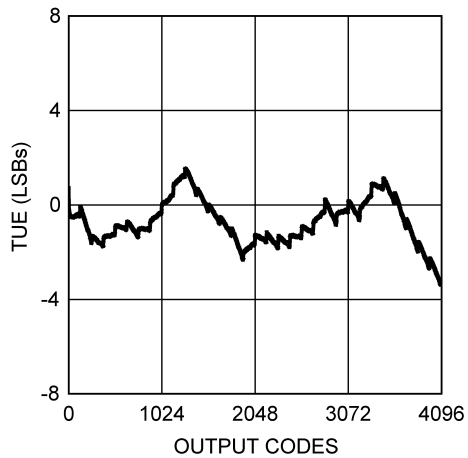
Figure 7. TUE at V_A = 3 \text{ V}
