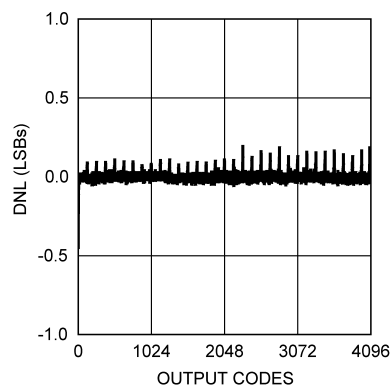
DNL vs. Output Code
