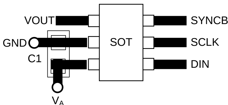
Figure 46. Typical Layout
