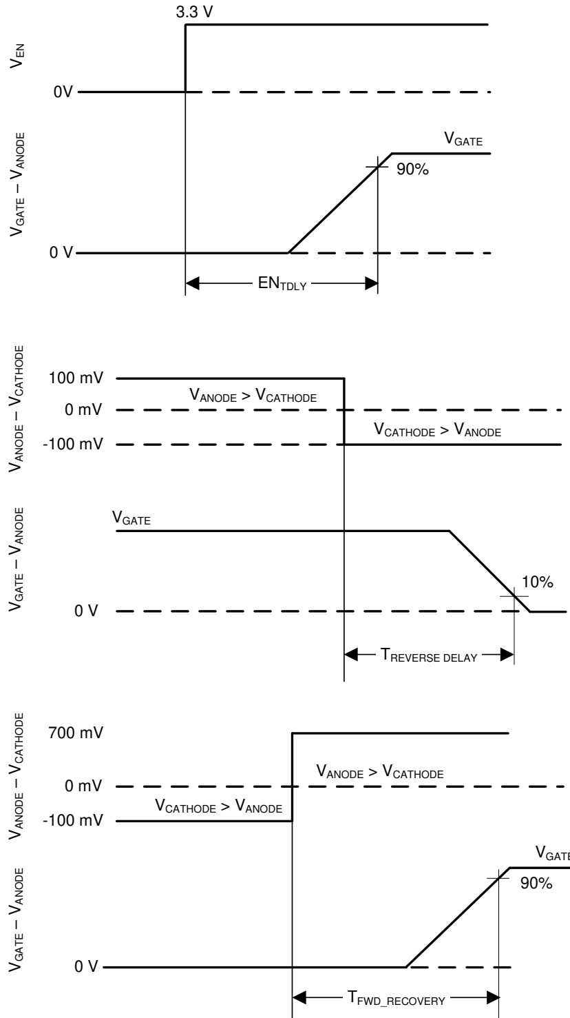
图 8-1. Timing Waveforms
