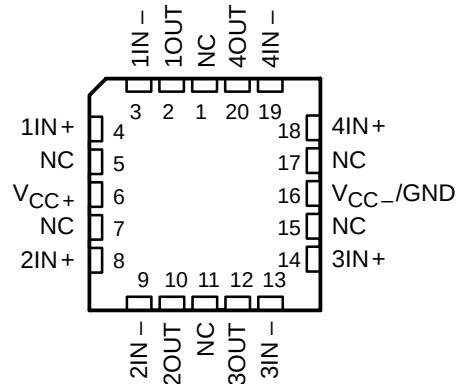
TLC2264M, TLC2264AM . . . FK PACKAGE (TOP VIEW)
