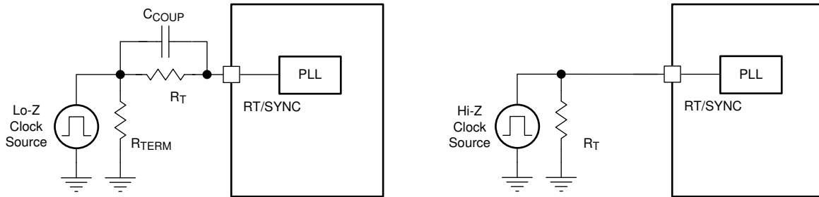
图 7-5. Synchronizing to an External Clock
