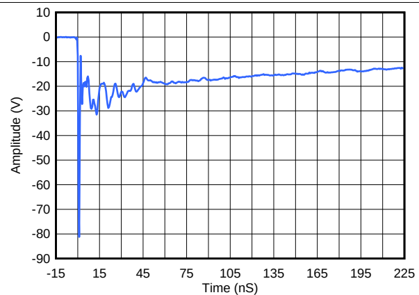
Figure 12. ESD Clamp Voltage -8\text{-kV} Contact ESD
