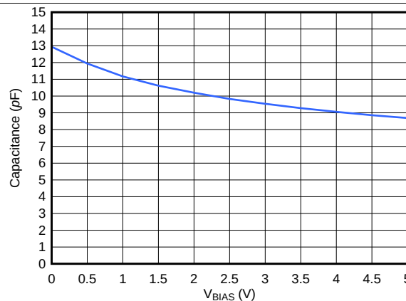
Figure 8. Pin Capacitance Across V_{BIAS}
