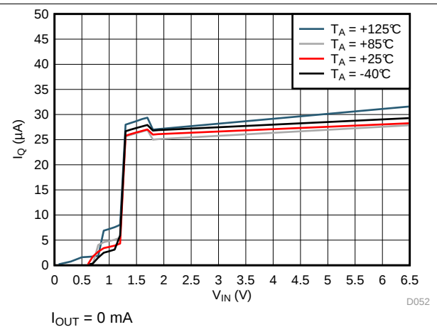
Figure 12. LP5912-1.8 I_Q (No Load) vs V_{IN}
