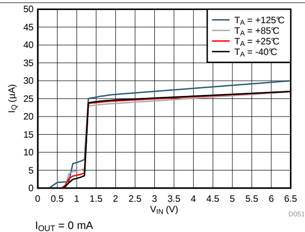
Figure 11. LP5912-0.9 I_Q (No Load) vs V_{IN}
