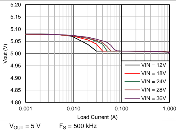
Figure 9. V_{OUT} Regulation
