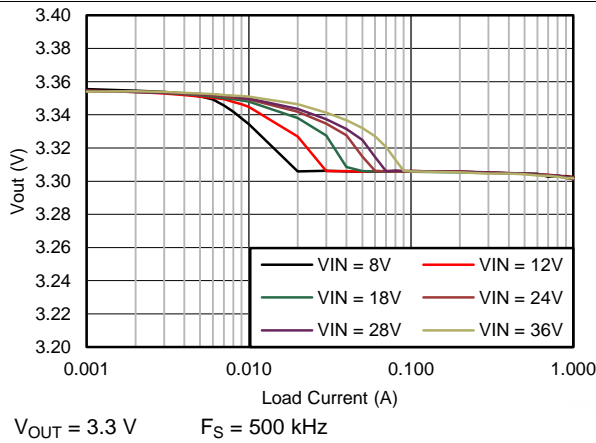
Figure 7. V_{OUT} Regulation
