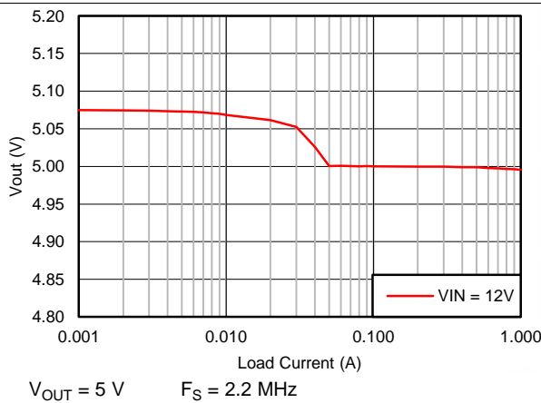
Figure 11. V_{OUT} Regulation
