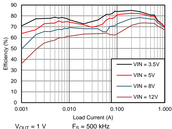
Figure 48. Efficiency
