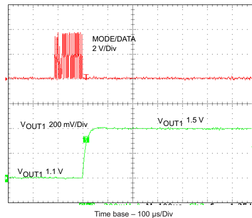
Figure 33. Typical Operation
