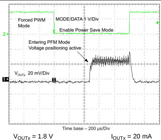
Figure 26. Forced PWM-to-PFM Mode Transition
