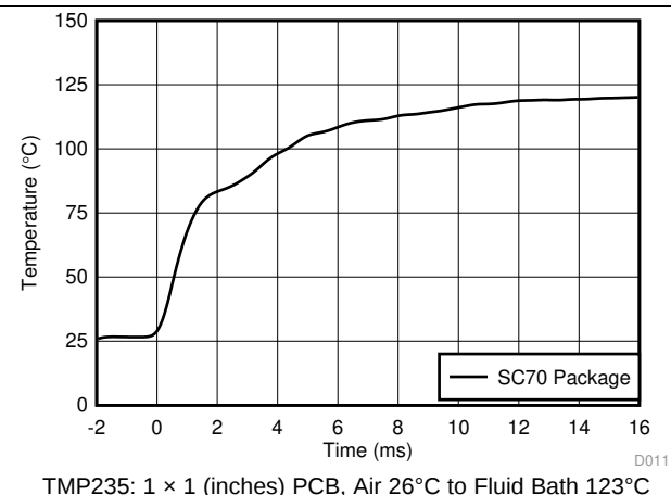
图 11. Thermal Response (Air-to-Fluid Bath)
