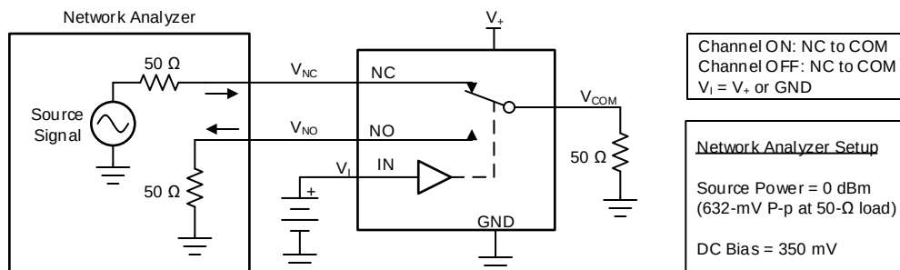
Figure 22. Crosstalk ( X_{Talk} )
