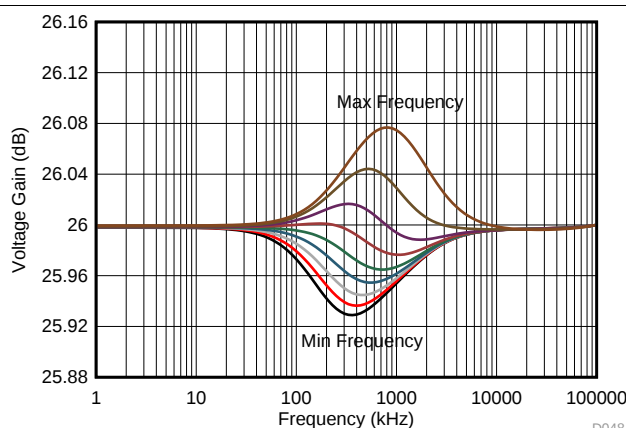
Figure 62. Thermal Frequency Control Sweep (Gain = 10)
