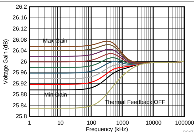
Figure 61. Thermal Gain Control Sweep (Frequency = 9)
