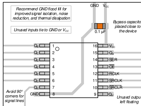
Figure 11-1. Example layout for the SN74HCS596.
