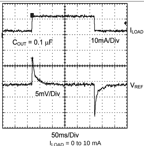
Figure 9. Load Transient Response
