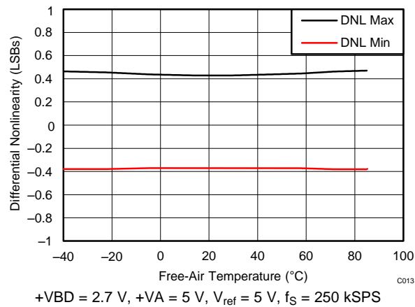
Figure 13. DNL vs Free-Air Temperature
