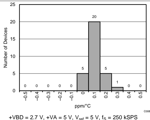
Figure 8. Offset Error Drift Histogram
