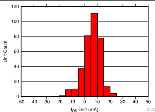
图 9-3. Input-Referred Offset Drift After AEC-Q100 High Temperature Operating Life Stress Test
