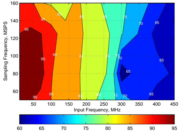
Figure 139. Spurious-Free Dynamic Range (SFDR) for 0-dB Gain
