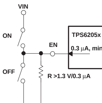
Figure 3. Pushbutton Configuration for the EN-Pin
