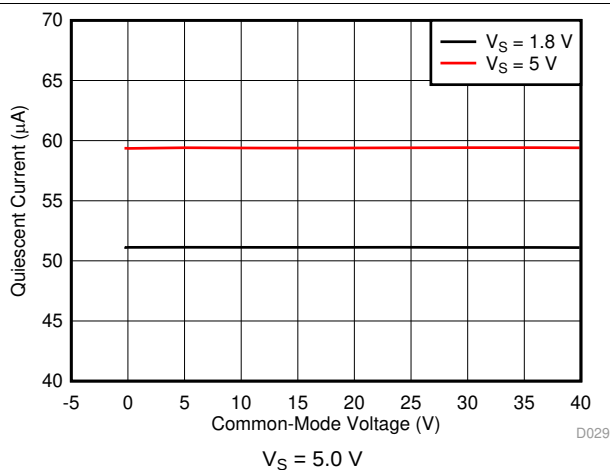
图 10. Quiescent Current vs Common Mode Voltage
