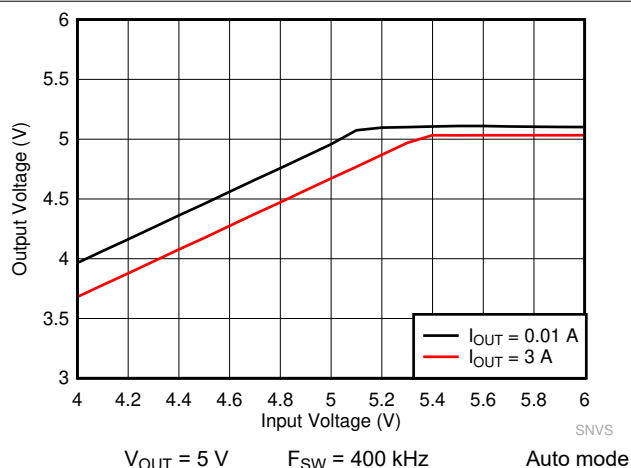
图 9-22. LM61430-Q1 Dropout Curve
