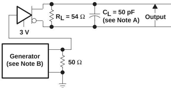
TEST CIRCUIT
