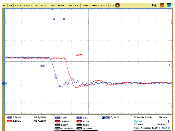
图 29. Typical Turnoff Waveform (CL = 1.8 nF, VDD = 12 V)
