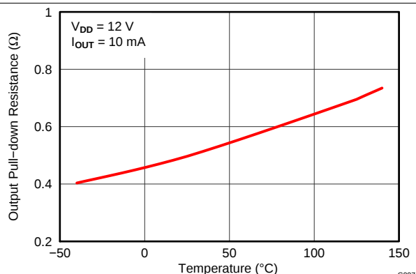
图 10. Output Pulldown Resistance vs Temperature
