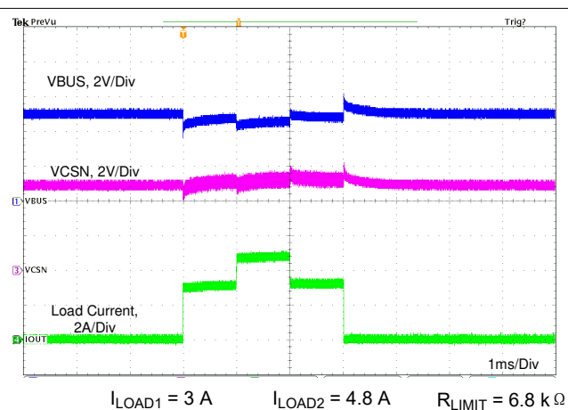
图 11-31. MFI Over-Current Test With External FET
