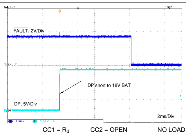
图 11-39. DP Short to BAT
