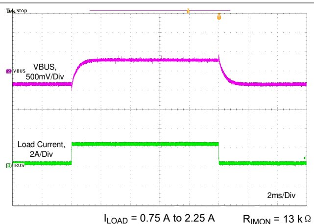
图 11-11. Load Transient with Cable Compensation
