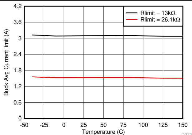
图 8-13. Buck Average Current Limit vs Junction Temperature
