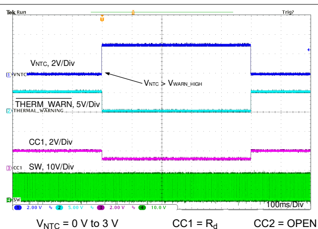
图 11-41. Thermal Sensing with NTC Behavior 1
