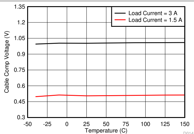
图 8-17. Cable Compensation Voltage vs Junction Temperature
