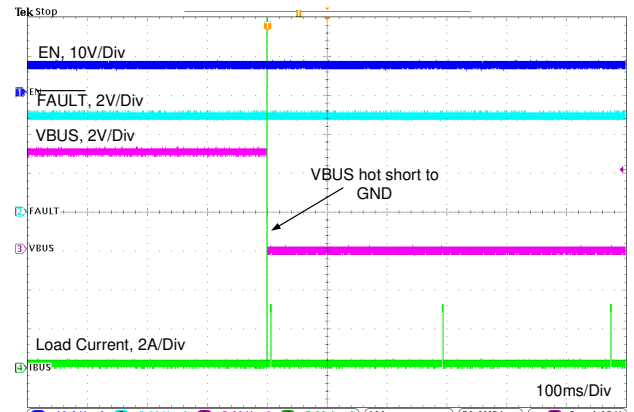
图 11-33. VBUS Hot Short to GND with External FET
