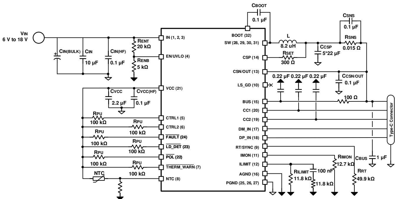
图 11-1. Application Circuit
