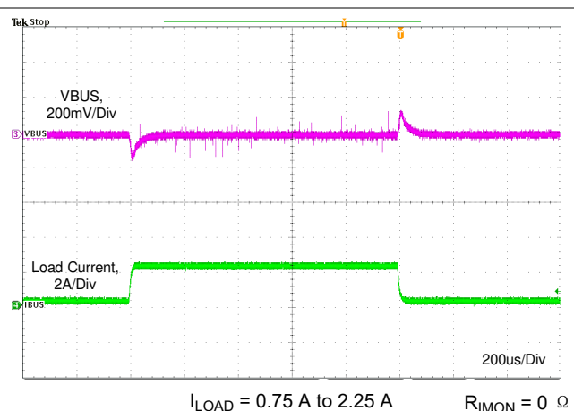
图 11-9. Load Transient Without Cable Compensation
