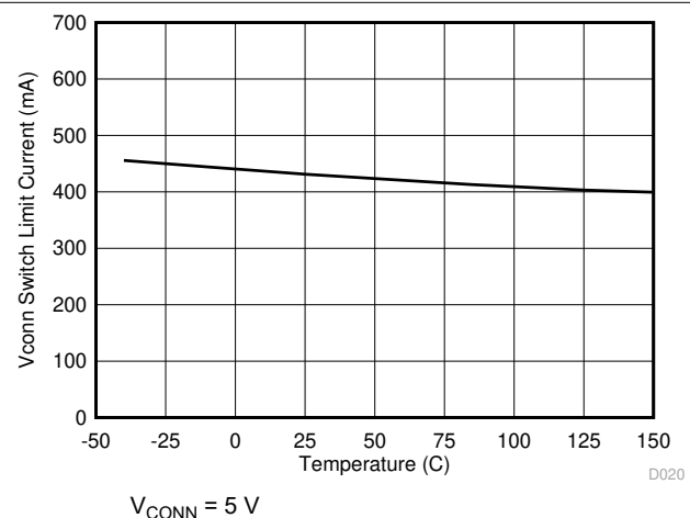
图 8-24. V CONN Switch Current Limit vs Junction Temperature
