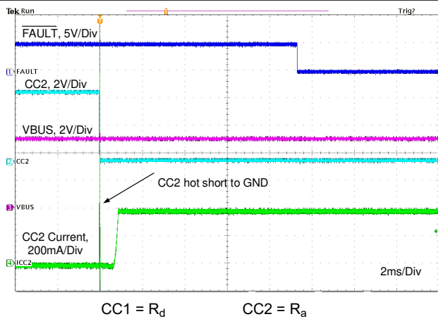
图 11-34. CC2 Hot Short to GND
