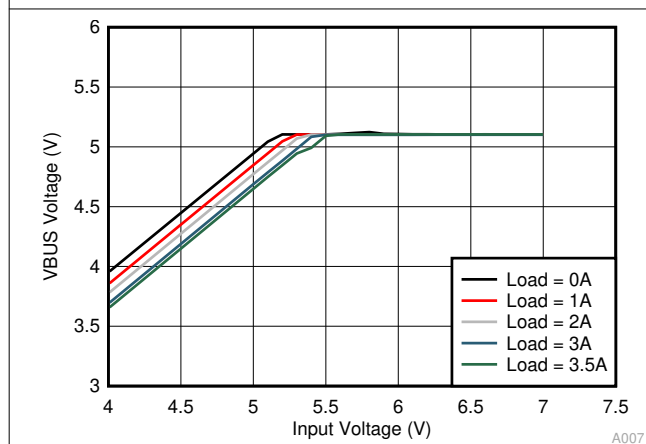
图 11-12. Dropout Characteristic
