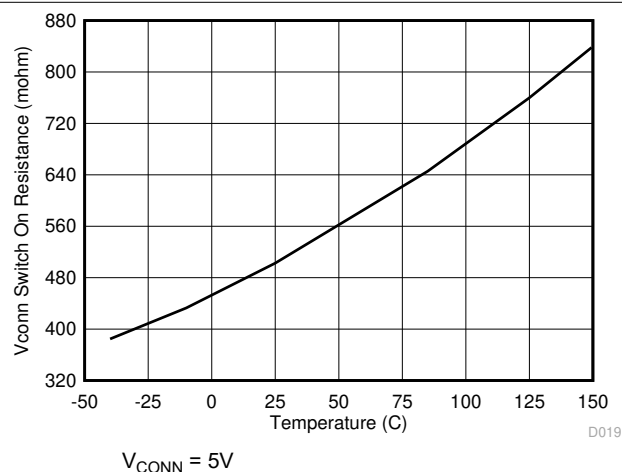
图 8-23. V CONN Current Limiting Switch On Resistance vs Junction Temperature
