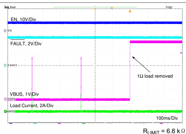
图 11-29. 1-Ω Load Recovery With External FET
