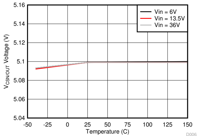
图 8-7. V_{CSN/OUT} Voltage vs Junction Temperature
