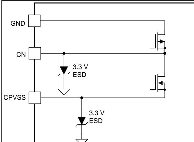
Figure 17. CN and CPVSS Pins
