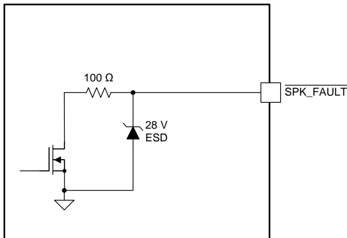
Figure 19. SPK_FAULT Pin
