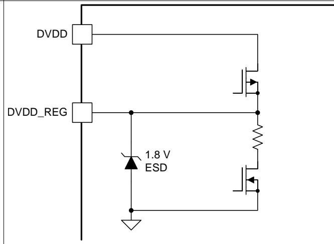
Figure 18. DVDD_REG Pin
