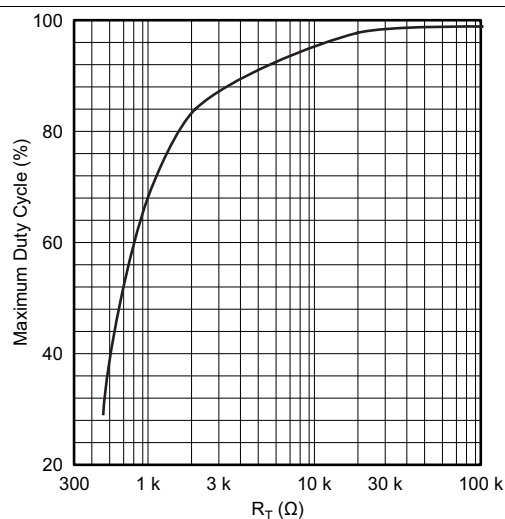
Figure 7. Maximum Duty Cycle vs Timing Resistance
