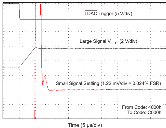
Figure 33. Half-Scale Settling Time, Rising Edge
