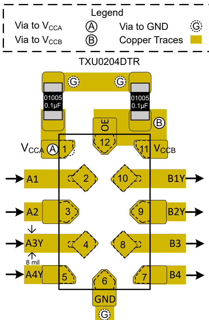
Figure 12-1. Layout Example – TXU0204
