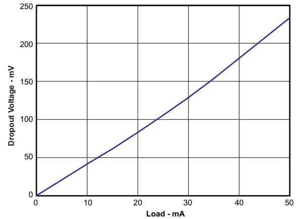
图 10. LDO Dropout Voltage vs Load Current
