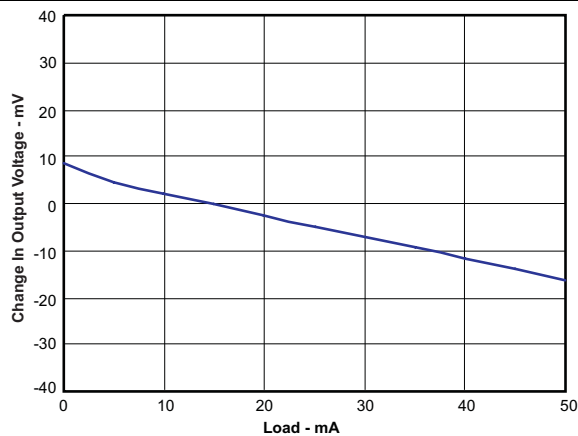
图 11. LDO Load Response
