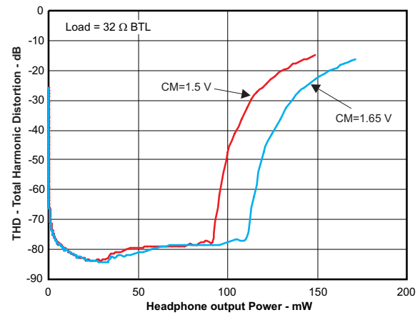
图 8. Total Harmonic Distortion vs Headphone Output Power
