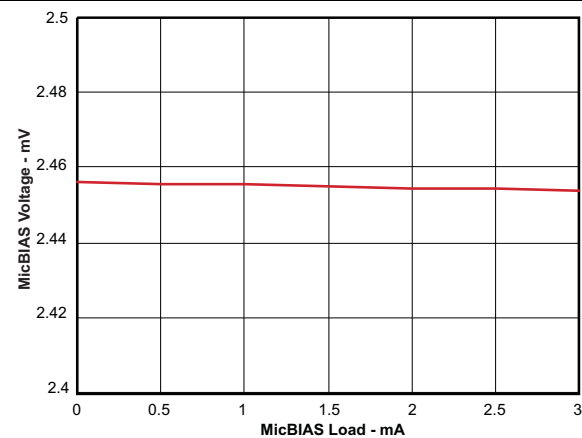
图 12. MICBIAS Mode 2, CM = 0.9 V, LDOIN OP Stage vs MICBIAS Load Current
