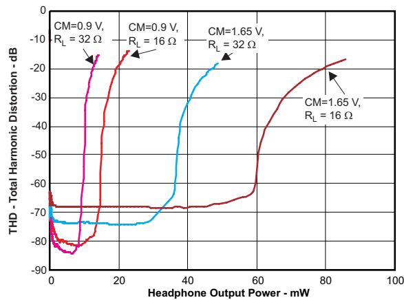
图 7. Total Harmonic Distortion vs Headphone Output Power
