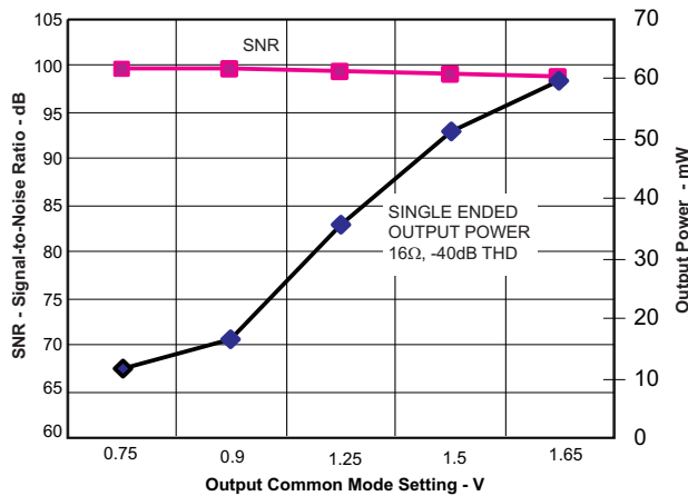
图 9. Headphone SNR and SE Output Power vs Output Common Mode Setting
