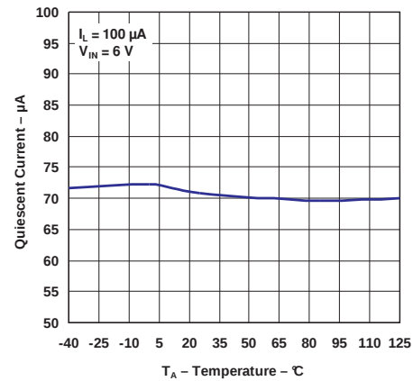
Figure 10. Quiescent Current vs Temperature ( I_L = 100 \text{ } \mu\text{A} )
