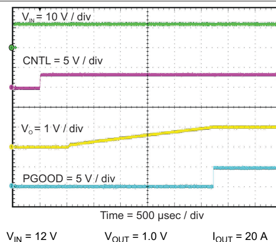
图 8-5. Start-Up from EN/UVLO
