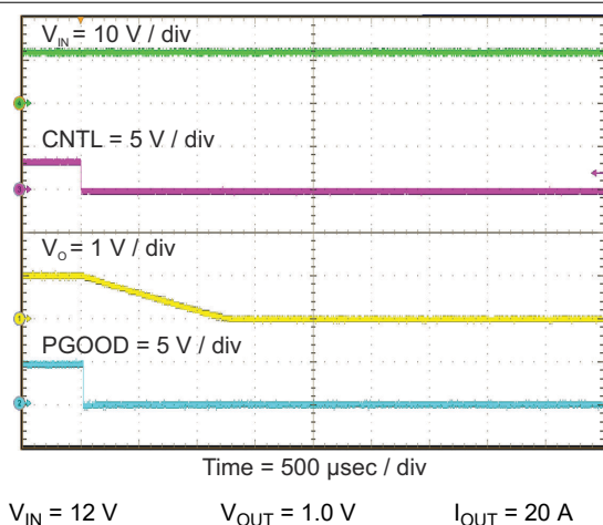
图 8-6. Shutdown from CNTL
