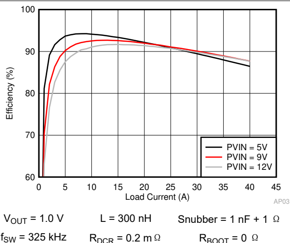
图 8-2. Efficiency vs Output Current
