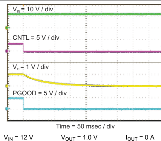
图 8-7. Shutdown from CNTL
