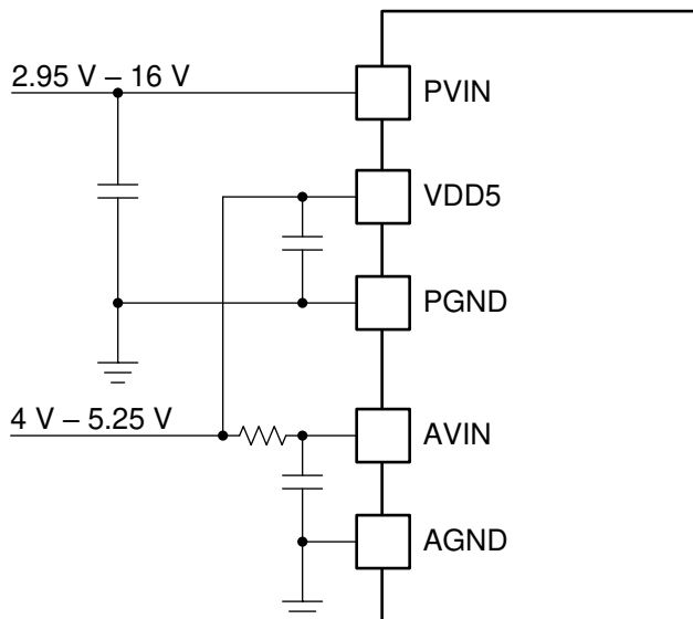
图 7-3. TPS546D24A Separate PVIN and AVIN connections with VDD5
